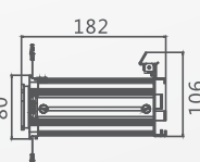
Zoom barrel (19°-36°) (68131000043)
